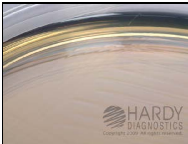
Proteus mirabilis (ATCC® 12453) growth inhibited on AnaeroGRO™ Bacteroides Bile Esculin Agar (Cat.
